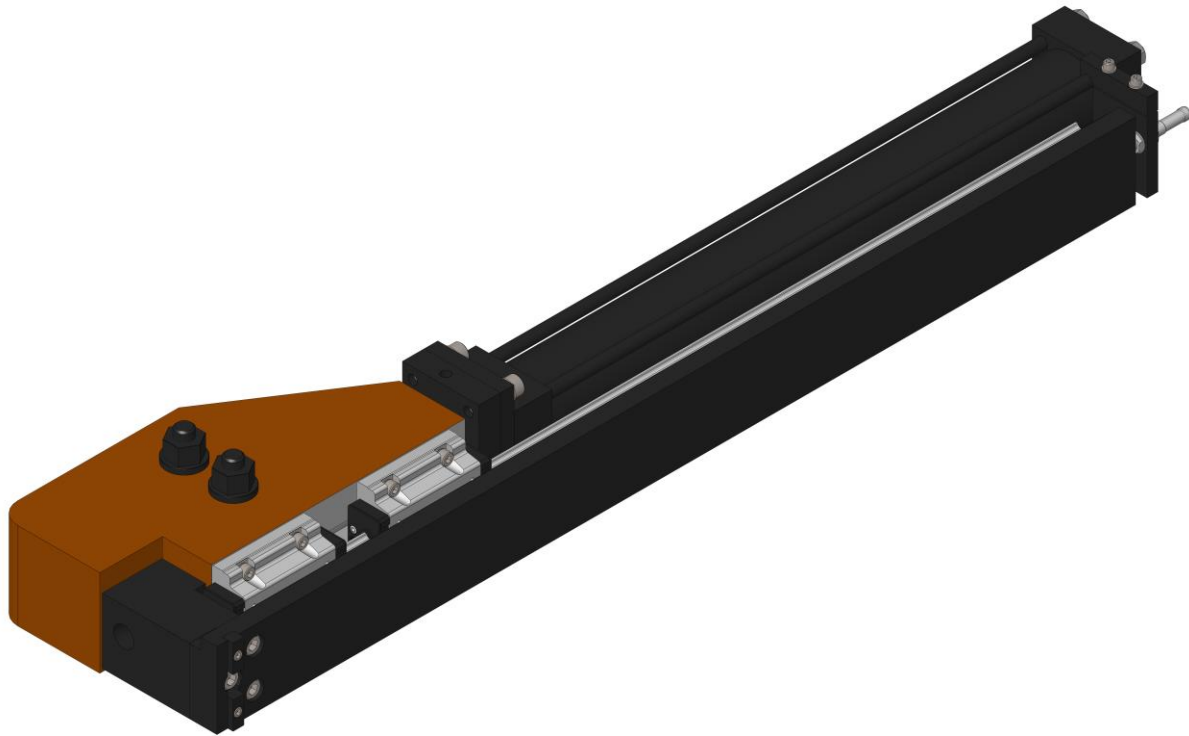
SUPERIOR USA ASSEMBLY PART NO. 30052-34600 (LH) or 30053-34600 (RH) for PINES #1 ¼ or #2 PRESSURE DIE ASSIST (PDA) ASSEMBLY (LH w/ 24" STROKE SHOWN, 30" STROKE ALSO STD.)
