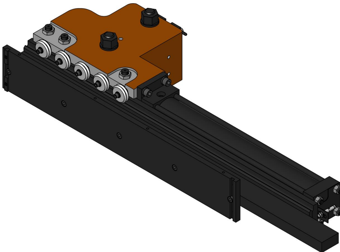
SUPERIOR USA ASSEMBLY PART NO. 60052-34600 (LH) or 60053-34600 (RH) for PINES #3 or #4 PRESSURE DIE ASSIST (PDA) ASSEMBLY (LH w/ 24" STROKE SHOWN, 30" STROKE ALSO STD.)
